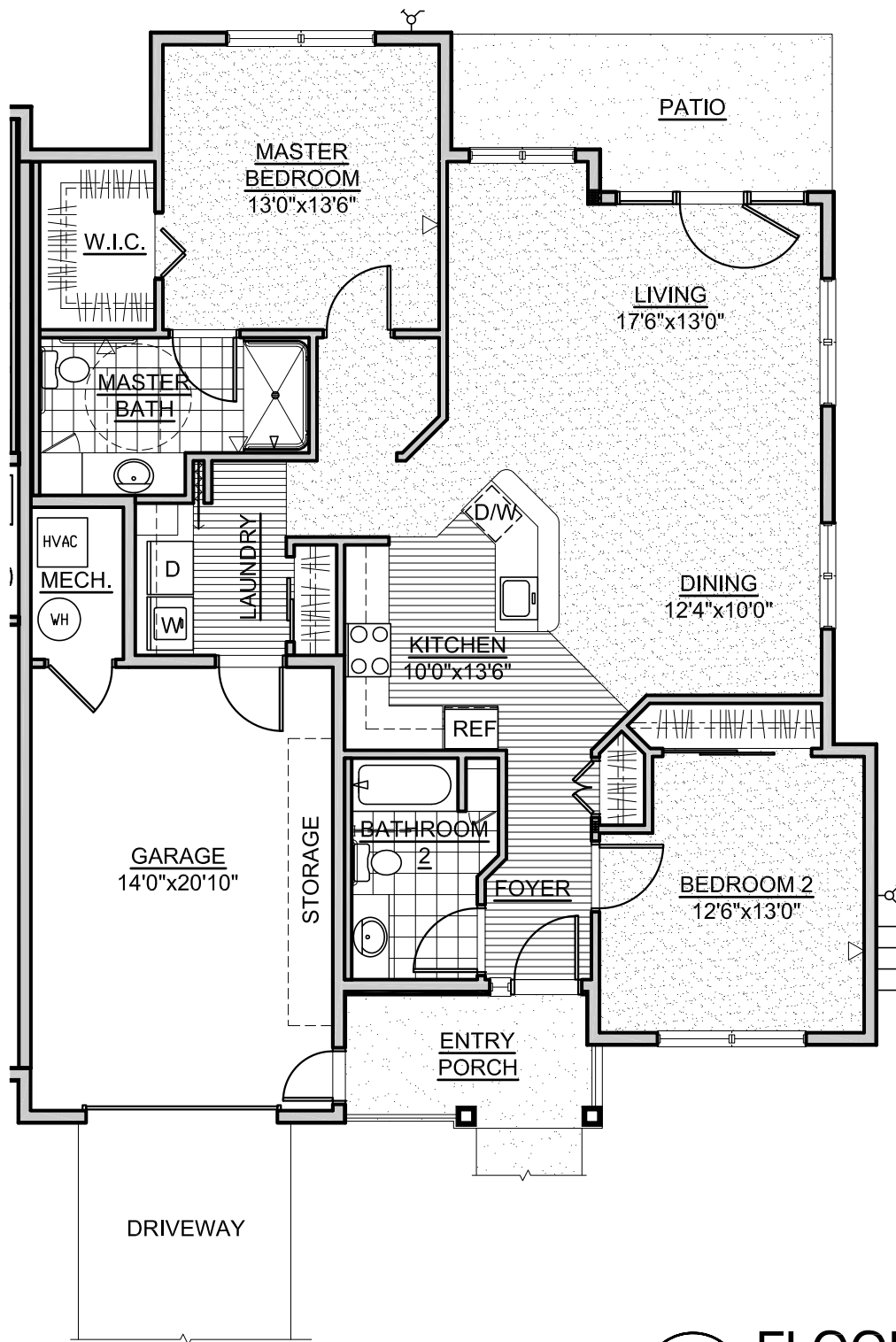
2 FLOOR PLAN (RIGHT UNIT 1/8"=1'-0") 0 4' 8' 16'
